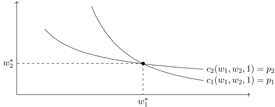
Figure 3.28: Candidate for equilibrium factor prices.
