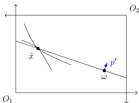
Figure 3.16: Non-equilibrium Pareto optimal allocation.
