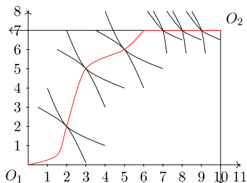
Figure 3.6: Pareto set that includes boundary allocations.
