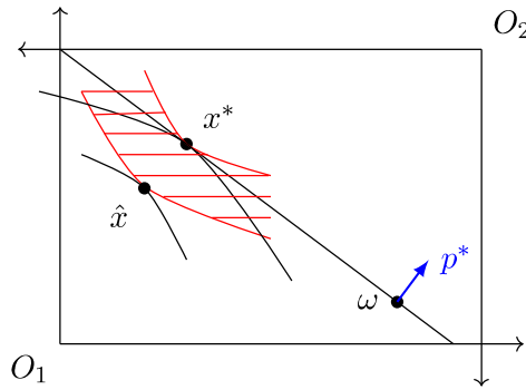
Figure 3.15: Non-Pareto optimal Walrasian equilibrium.
